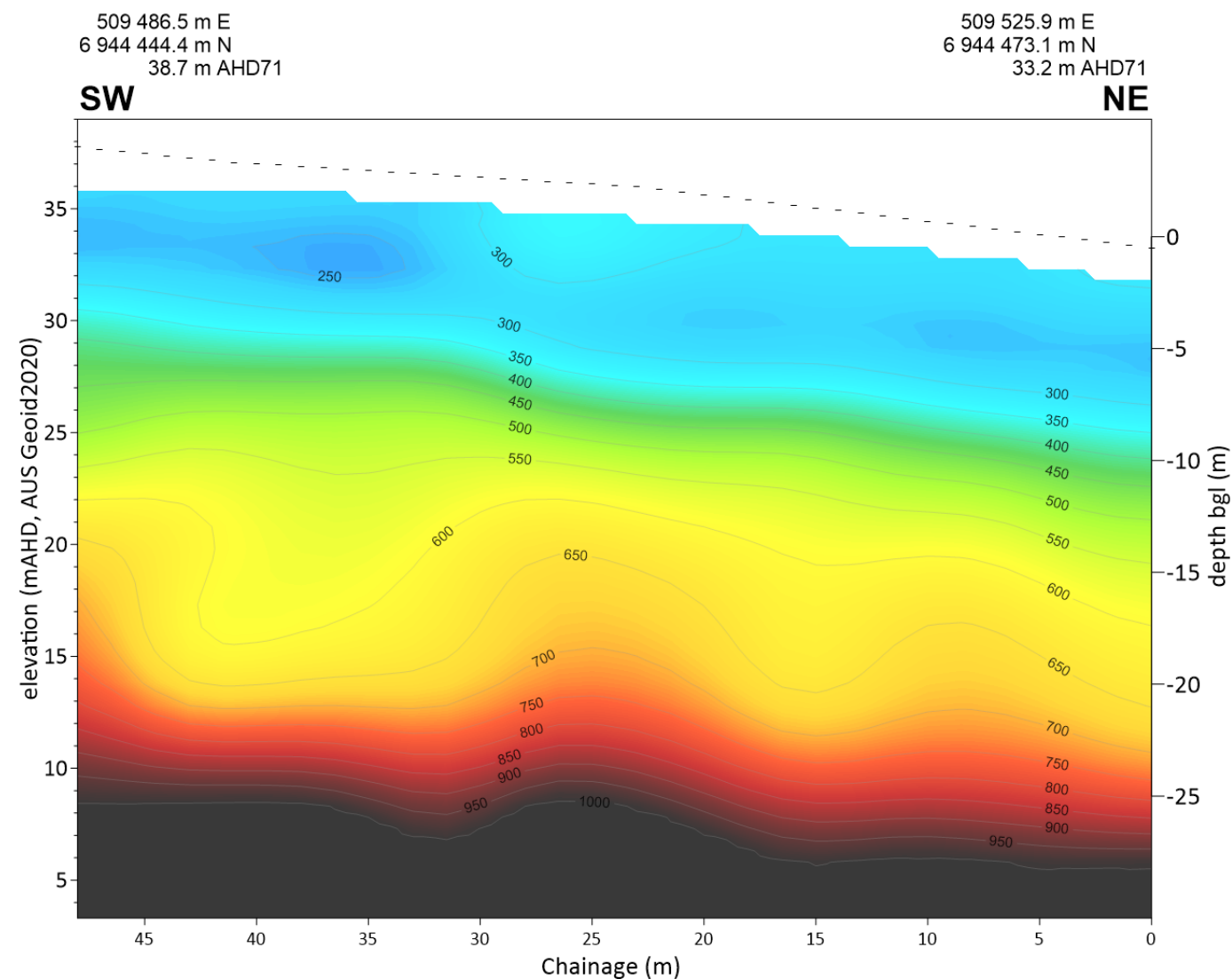
Seismic Line MASW AU-GP 119
